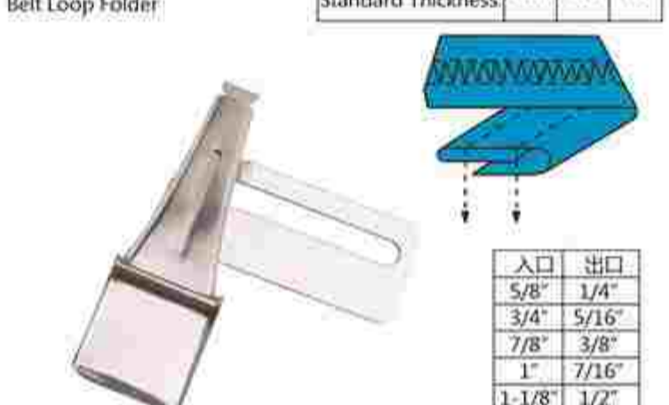
RX-G22 (F340) 耳仔筒 Belt Loop Folder
