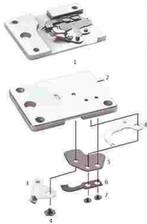
MB-377定刀剪线组件 ASSEMBLY FOR MB-377
