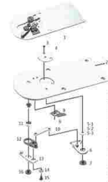
SPA/A-1306-HS剪线组件 ASSEMBLY FOR SPA/A-1306/HS
