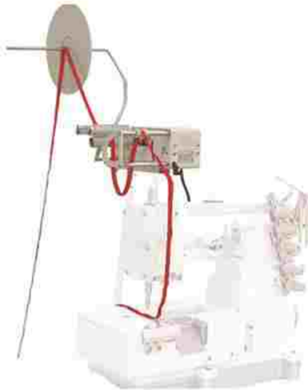
侧送型送料机送料宽度70mm side Tape Feeder, Feed Width 70mm
