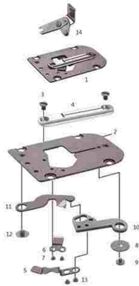
LBH-780剪线组件 ASSEMBLY FOR LBH-780
