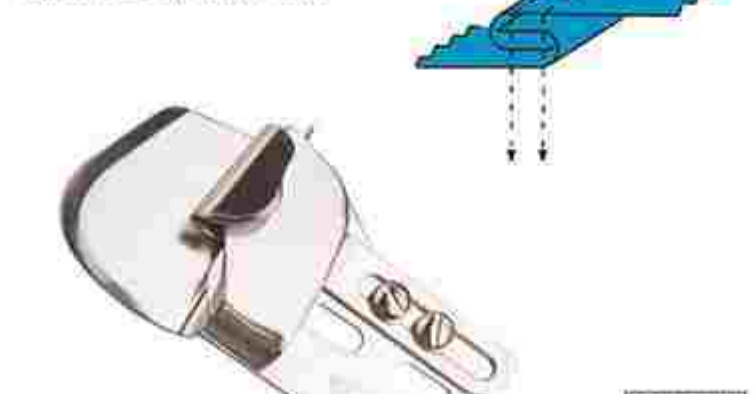
RX-G24 (F333) 双针上袖筒 Double Needle Lap Seam Folder
