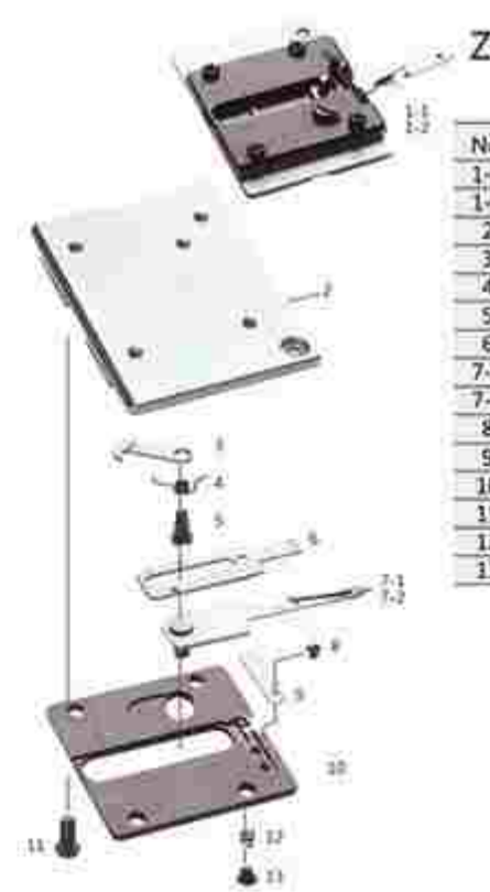
BROTHER/兄弟 ZE-8560A定刀剪线组件 ASSEMBLY FOR ZE-8560A
